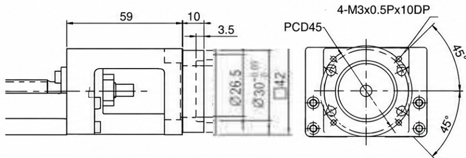
Motor Adaptor Flange F2
