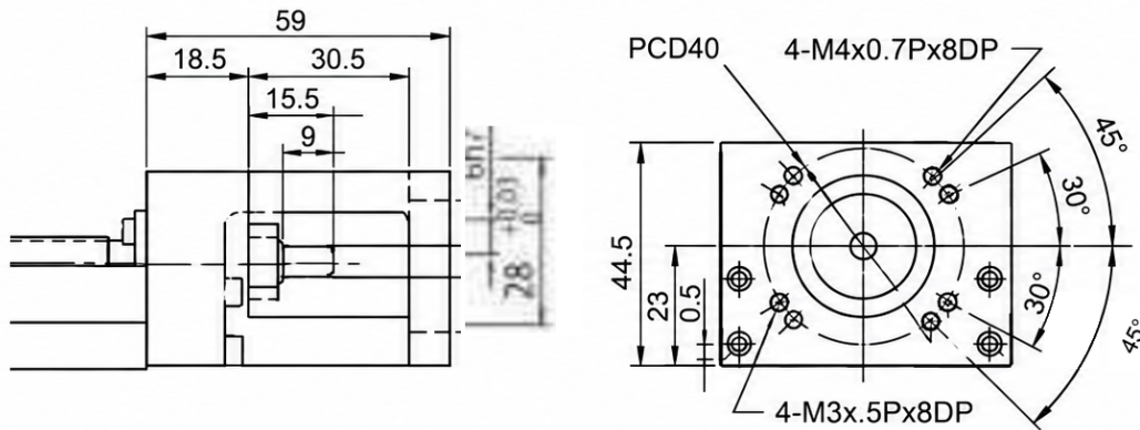
Motor Adaptor Flange F0
