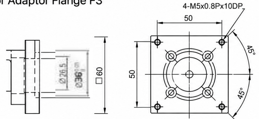
Motor Adaptor Flange F3
