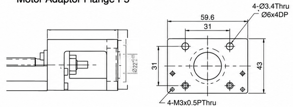
Motor Adaptor Flange F5
