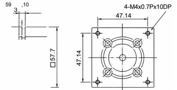
Motor Adaptor Flange F4
