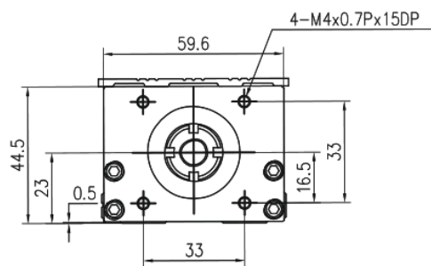
VIEW B
