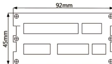
Rear panel size ( mm ) : 92X45
