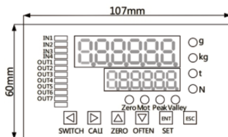
Front panel size ( mm ) : 107X60
