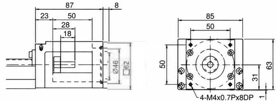
Motor Adaptor Flange F6
