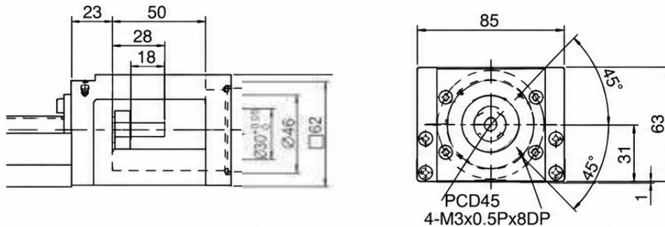
Motor Adaptor Flange F3
