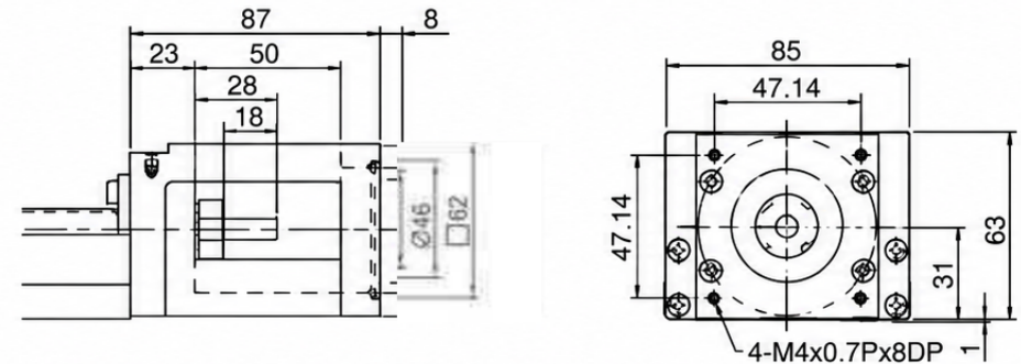
Motor Adaptor Flange F6
