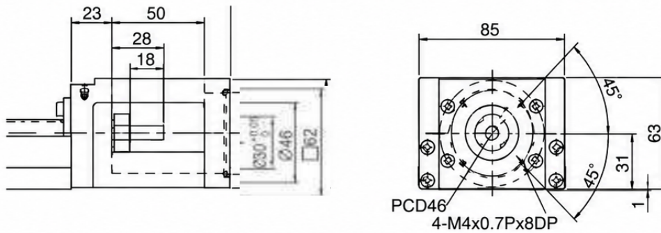
Motor Adaptor Flange F3
